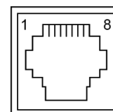
Złącze RS1 (RJ45)
