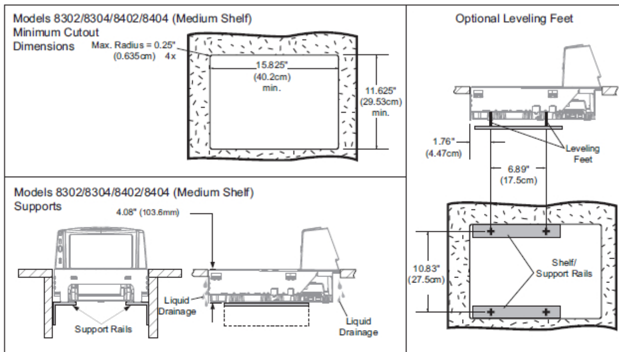
Figure 2-11. Medium Shelf Models 8302/8304/8402/8404 Cutout Dimensions
