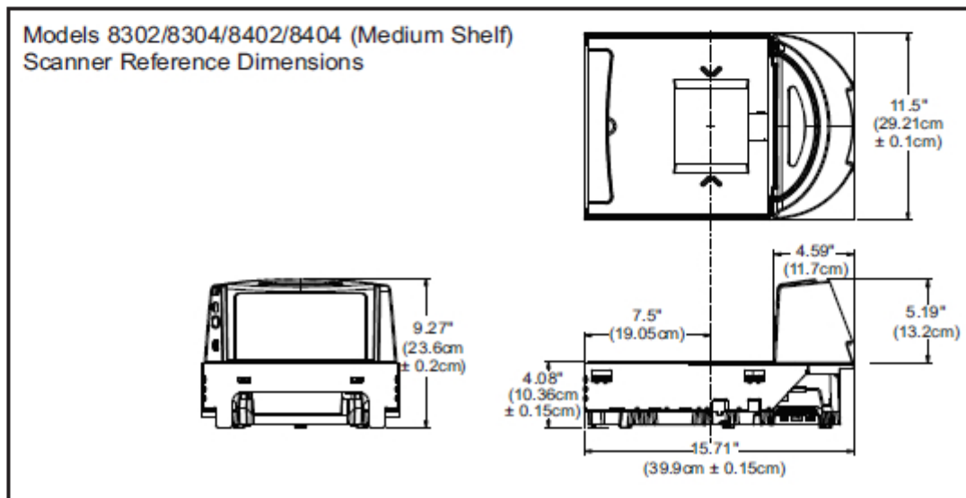
Figure 2-12. Medium Shelf Models 8302/8304/8402/8404 Scanner Reference Dimensions
